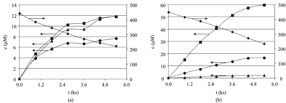
Fig. 1 (a) Photocatalytic oxidation of nitrobenzene: (◆) nitrobenzene, (●) 2-nitrophenol, (▲) 3-nitrophenol, (■) 4-nitrophenol. (b) Photocatalytic oxidation of N -phenylacetamide: (◆) N -phenylacetamide, (●) N -(2-hydroxyphenyl)acetamide, (▲) N -(3-hydroxyphenyl)acetamide, (■) N -(4-hydroxyphenyl)acetamide.
